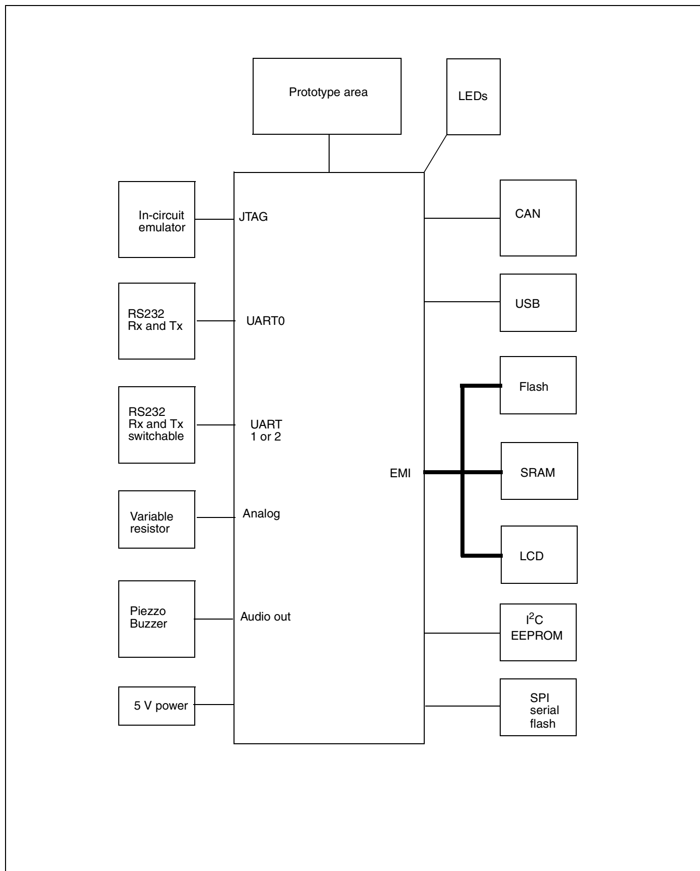
Figure 2: STR710-EVAL board system block diagram
