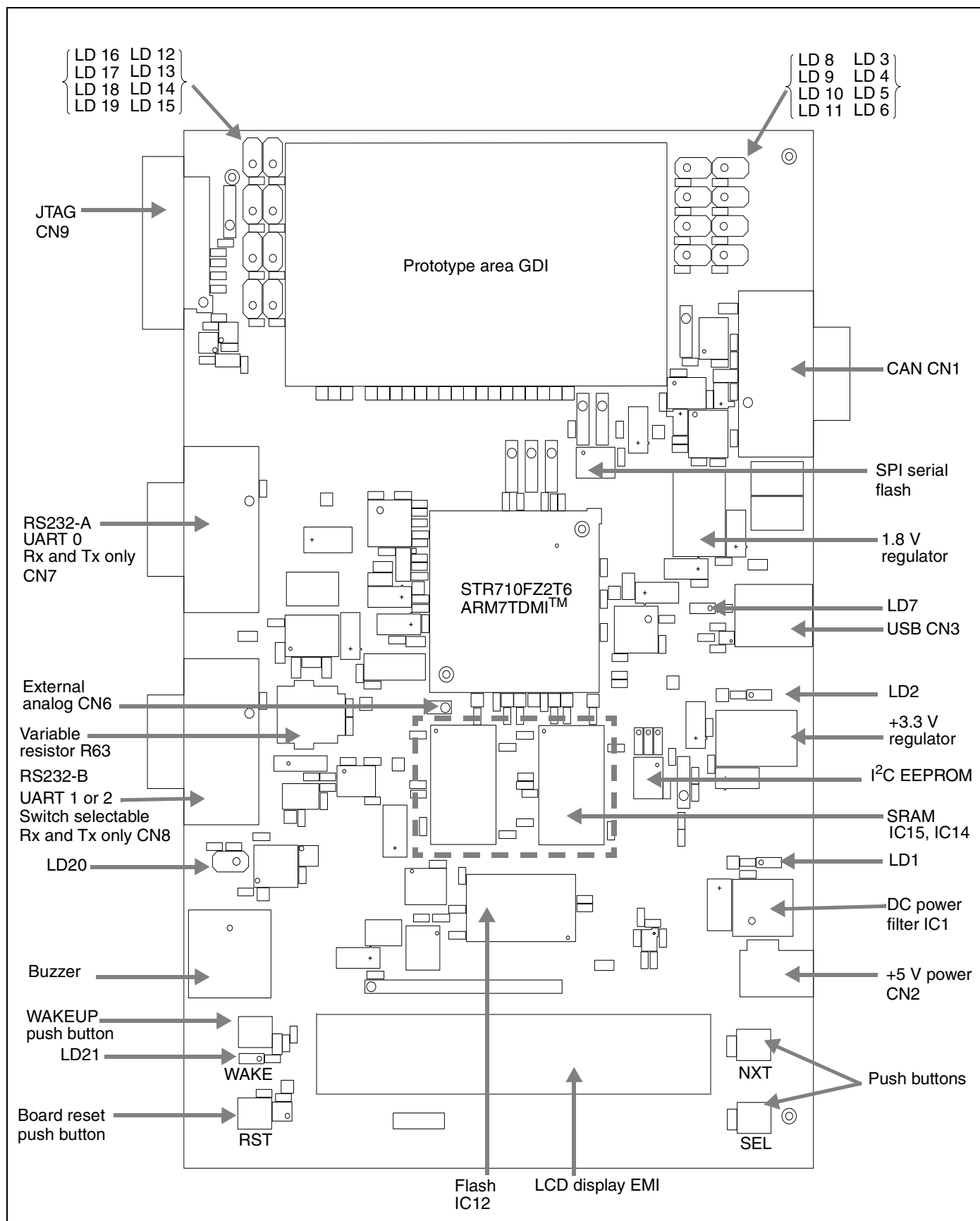
Figure 1: STR710-EVAL board layout block diagram
