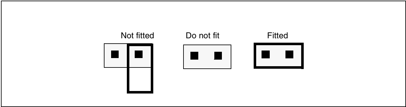
Figure 4: Jumper positions
